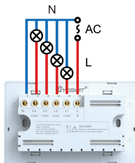
Connection 2: With neutral wire
